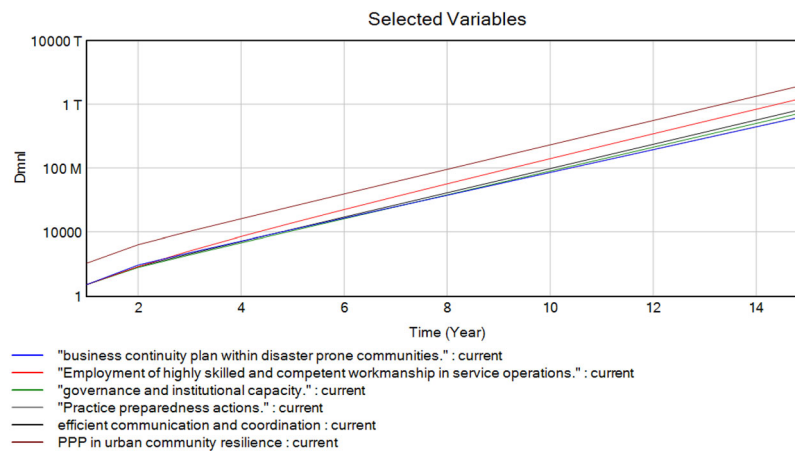
Figure 3. Simulation results for five (5) stock variables.
